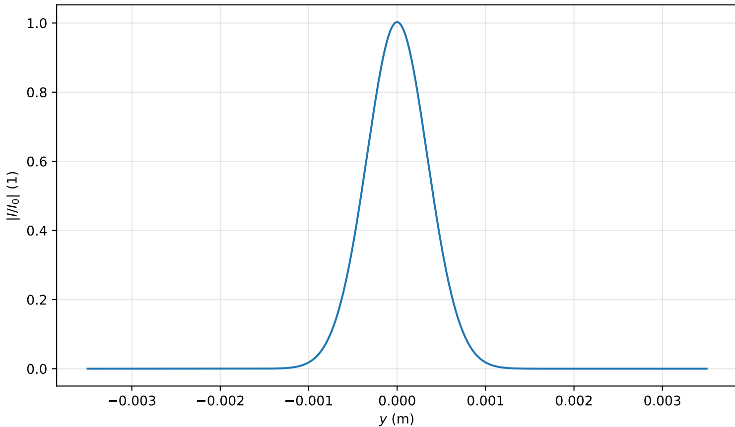
Intensity profile I(x=0, y, z=0.318)/I_0 , P_{in}=0.3P_{cr} , artificial time
